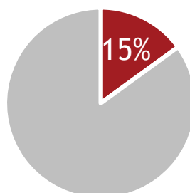
Hough
